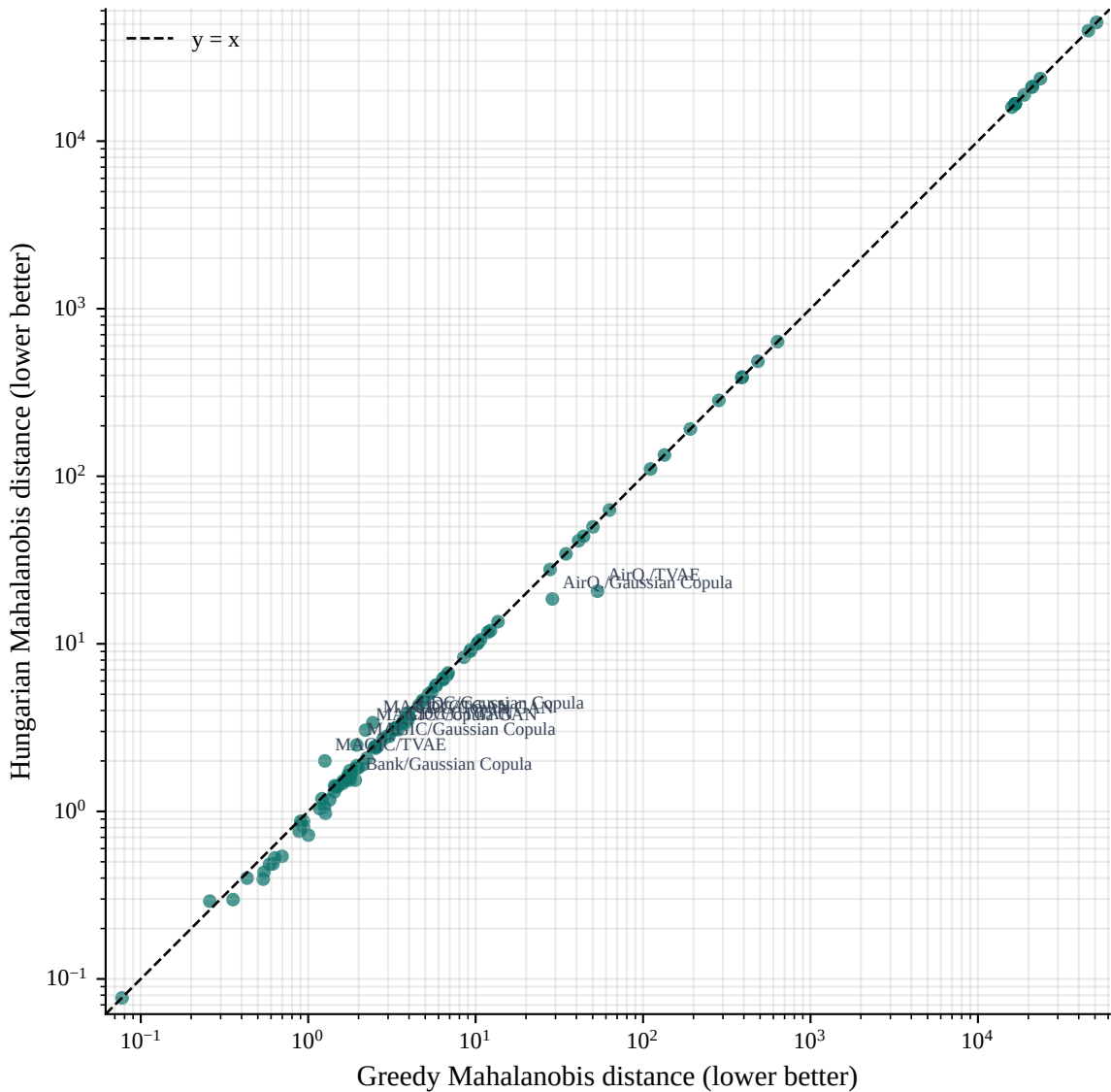
Greedy vs Hungarian Mahalanobis mapping
